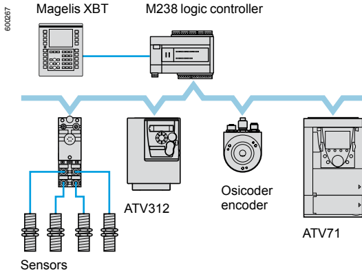
Configuration example on CANopen machine bus
