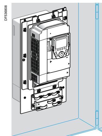
ATV71HU75N4 flush-mounted
