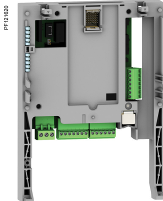
Extended I/O card VW3A3202
