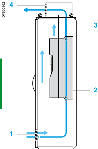
IP 23 cooling circuit
