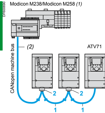
Optimized solution for daisy chain connection to the CANopen machine bus
